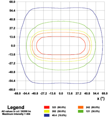
Iso Candela Diagram
