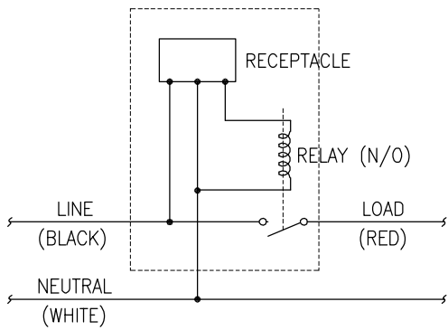
WIRING DIAGRAM
