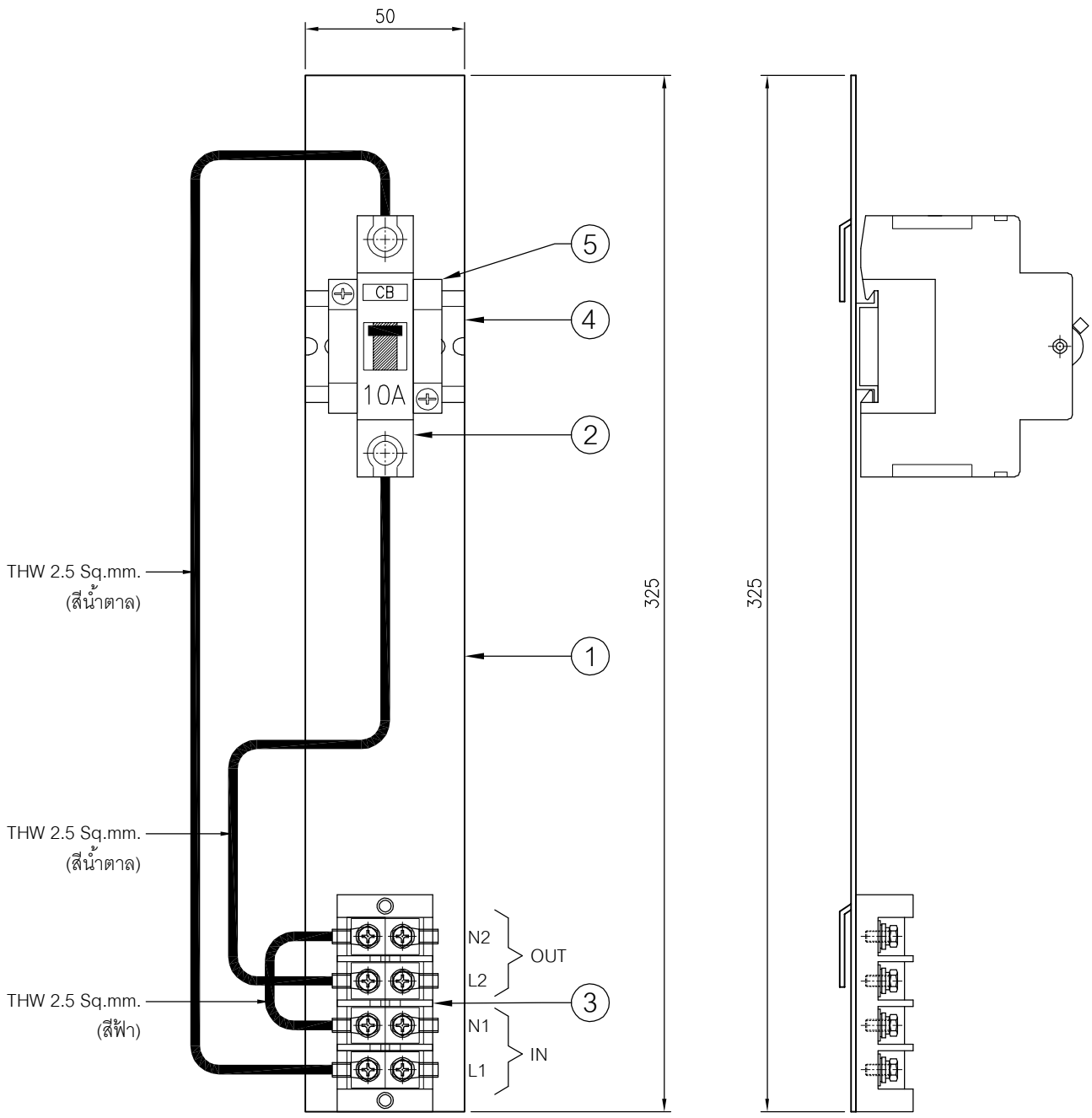
FRONT VIEW SCALE 1 : 2
