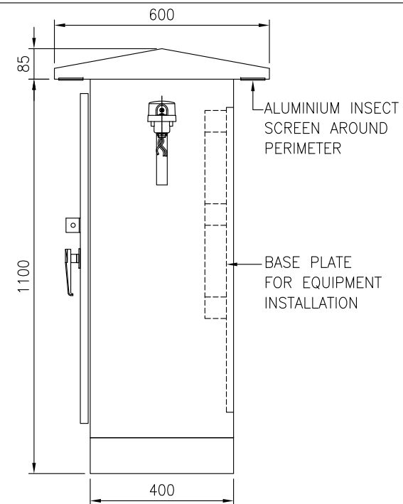
SIDE VIEW SCALE 1 : 15
