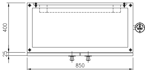
TOP VIEW SCALE 1 : 15
