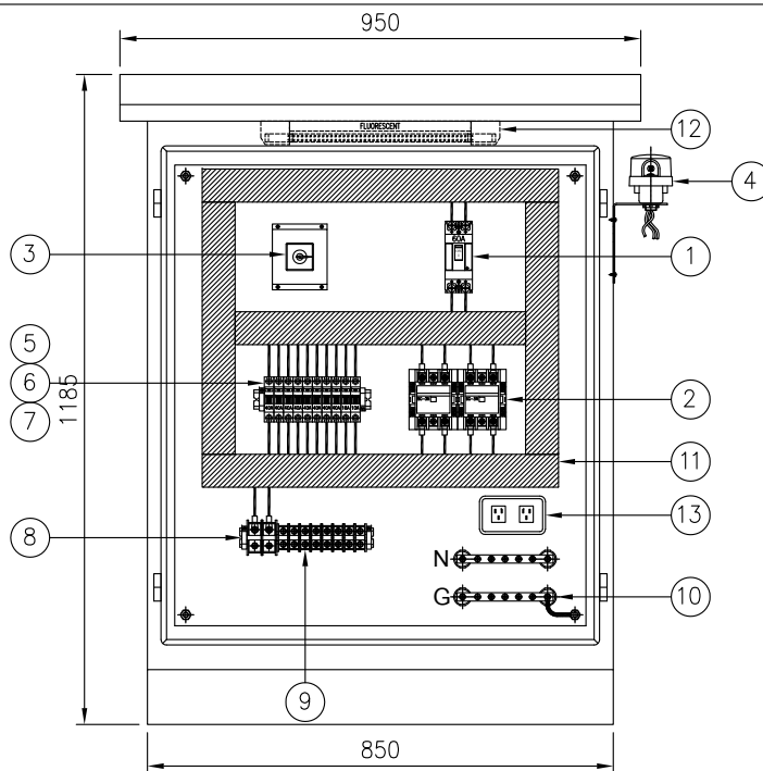
FRONT VIEW SCALE 1 : 15
