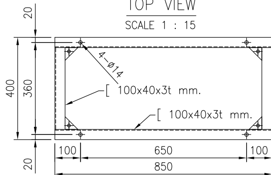
FOOTING FRAME DETAIL SCALE 1 : 15
